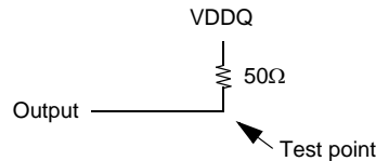
Figure 3 : Pulldown slew rate test load
