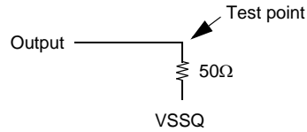
Figure 2 : Pullup slew rate test load
