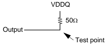
Figure 2 : Pulldown slew rate test load
