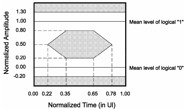
Mask of the eye diagram for the optical transmit signal
