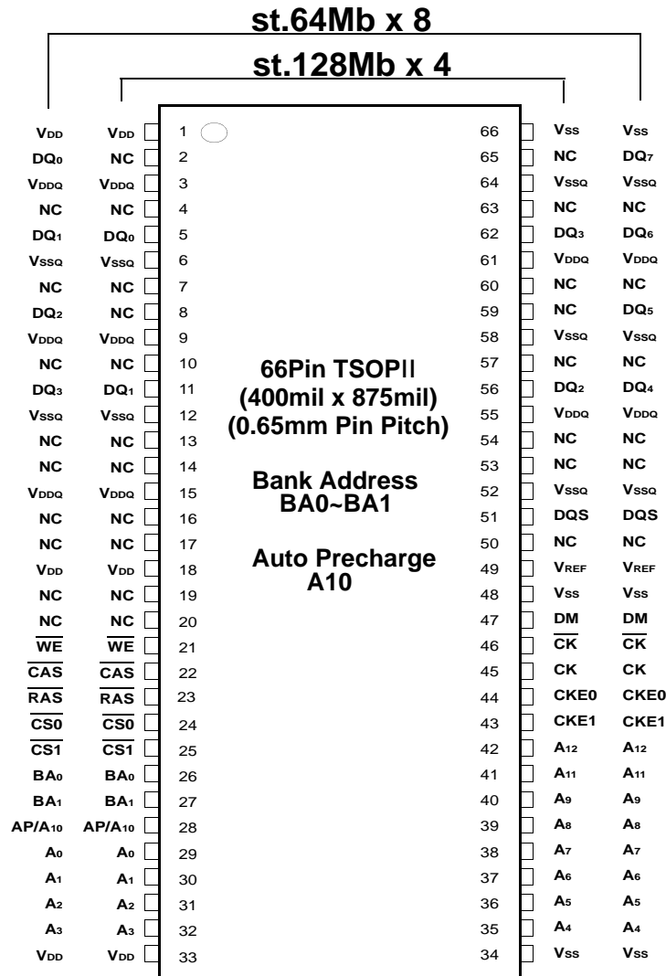
stacked 512Mb TSOP-II Package Pinout
