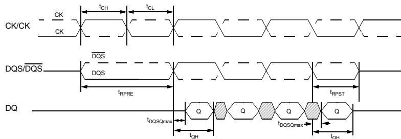
Figure 4 - Data Output (Read) Timing
