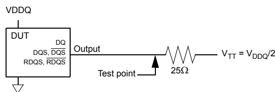
Figure 2 - Slew Rate Test Load
