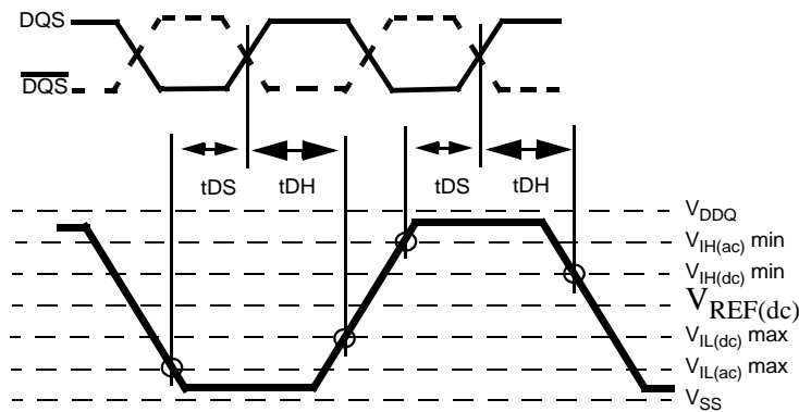
Differential Input waveform timing
