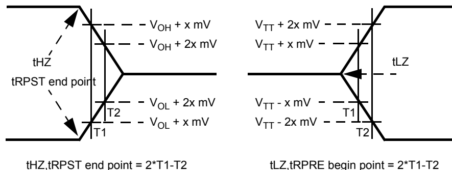
Figure 19. Method for calculating transitions and endpoints
