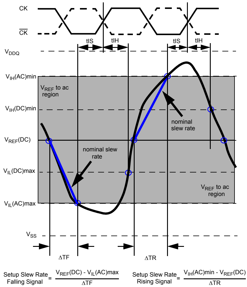
Figure 15. Illustration of nominal slew rate for tIS
