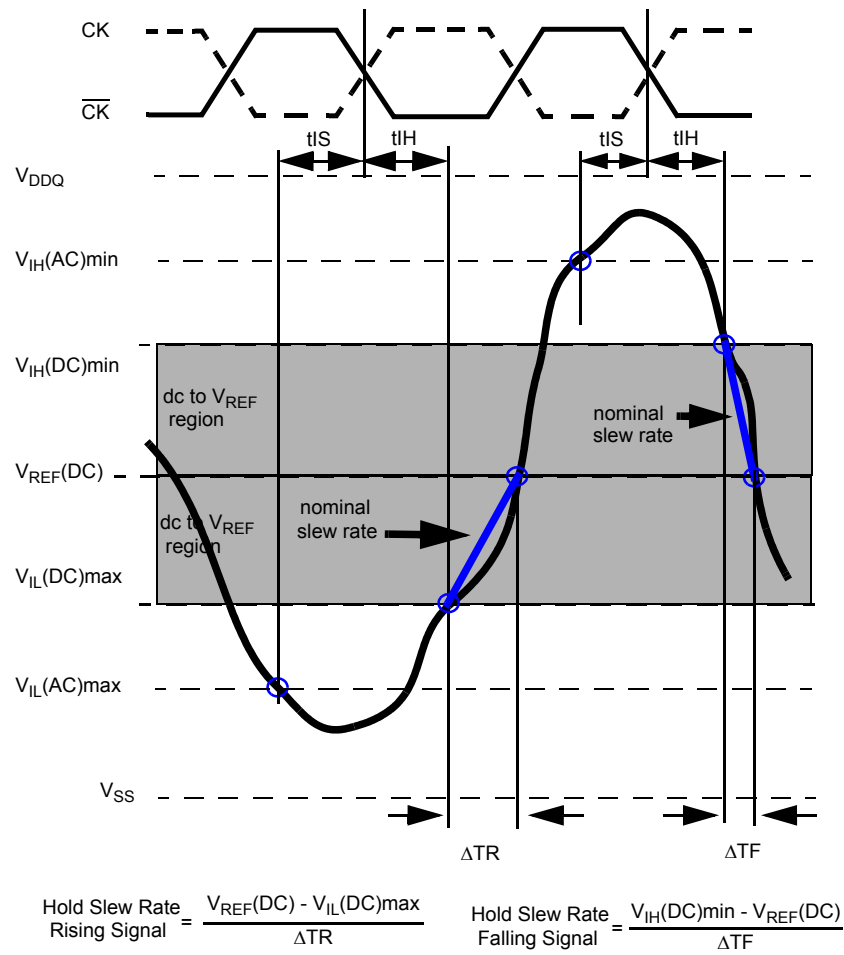
Figure 17. Illustration of nominal slew rate for tIH
