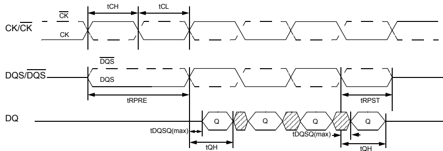
Figure 6. Data Output (Read) Timing
