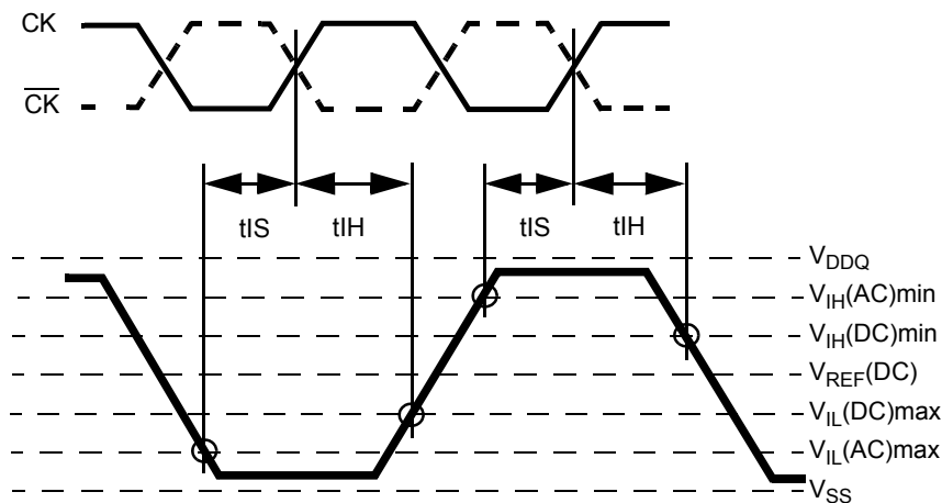
Figure 21. Differential input waveform timing - t_{IS} and t_{IH}
