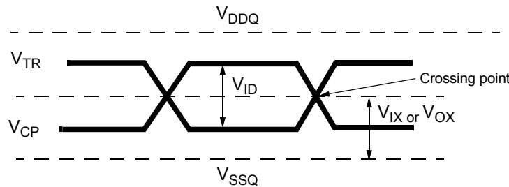
Figure 2. Differential signal levels
