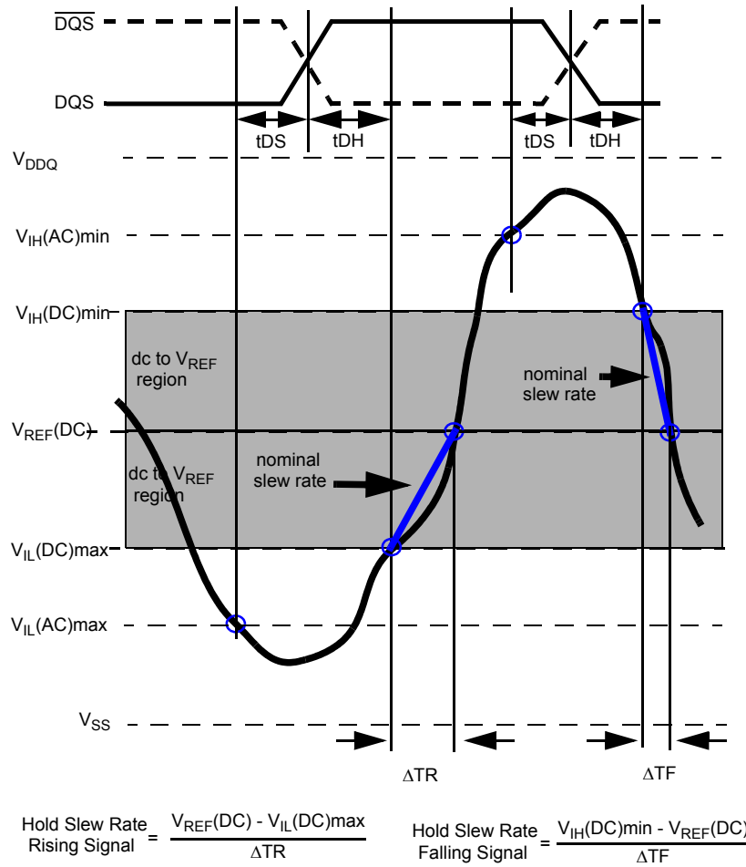
Figure 11. Illustration of nominal slew rate for t DH (differential QoS, \overline{DQS} )
