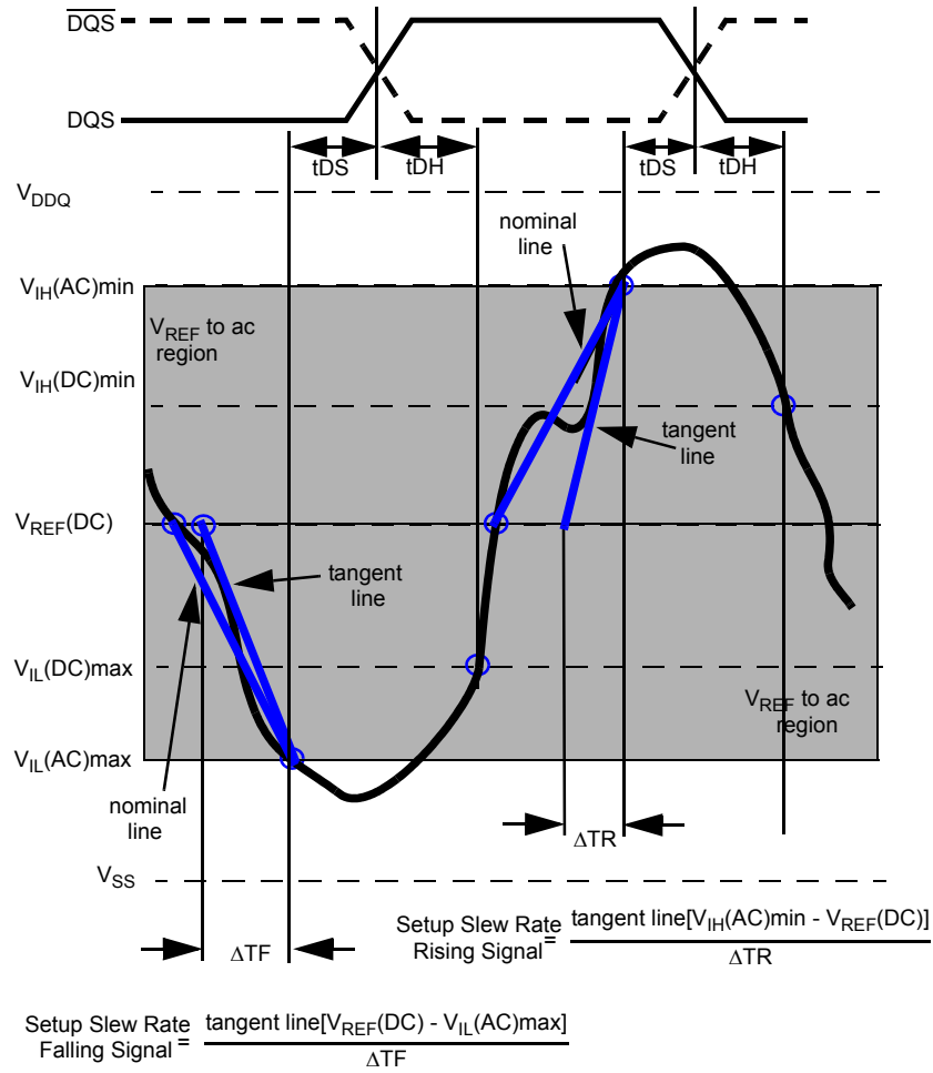
Figure 16. Illustration of tangent line for t1S
