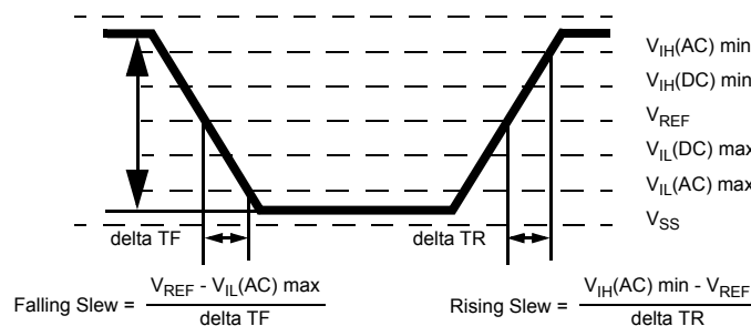
Figure 1. AC Input Test Signal Waveform
