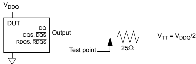
Figure 4. Slew Rate Test Load
