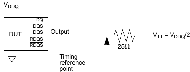
Figure 3. AC Timing Reference Load
