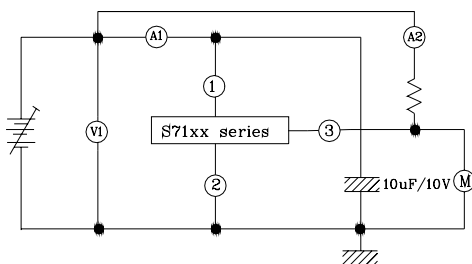
Test Circuit 1
