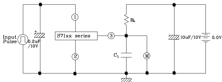
Test Circuit 2
