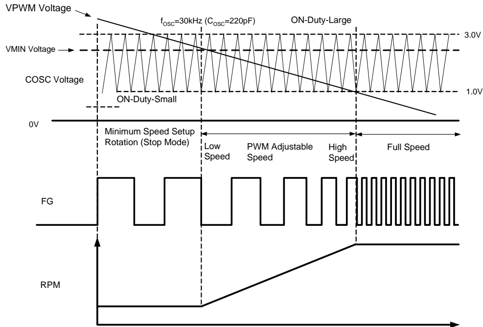
Figure 9. Operating Diagram 1 of AM4967 (Speed Control, Note 3)
