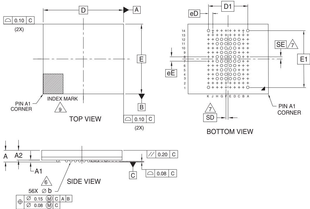
Figure 4.4 NLB056—56-ball VFBGA
