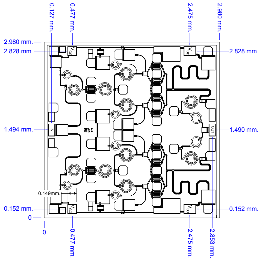
Figure 5. Die Layout
