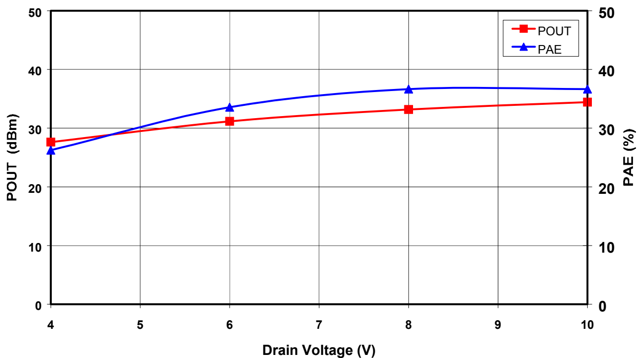
Figure 2. Saturated Output Power and Power Added Efficiency vs. Drain Voltage at f_o = 7.5 \text{ GHz} .
