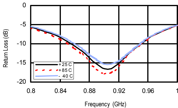
Input Return Loss vs Frequency (860 & 915 Band)
