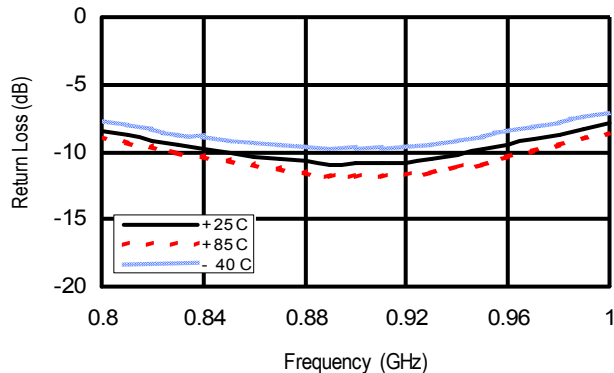
Output Return Loss vs Frequency (860 & 915 Band)
