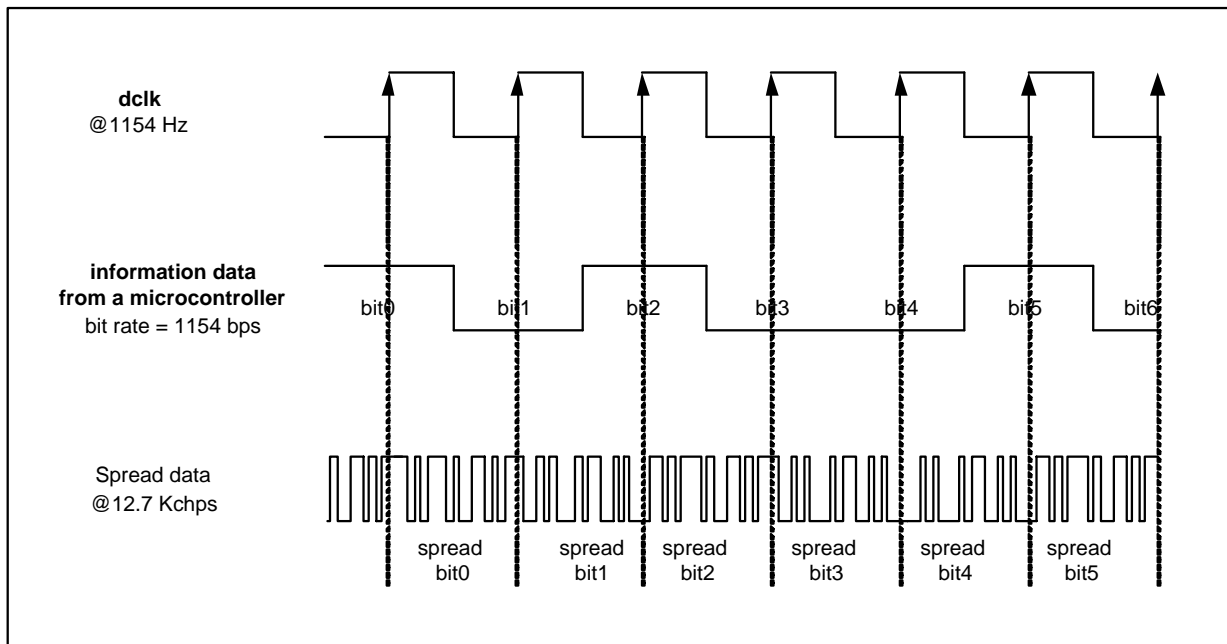
Figure 10 Data exchange during transmission mode.
