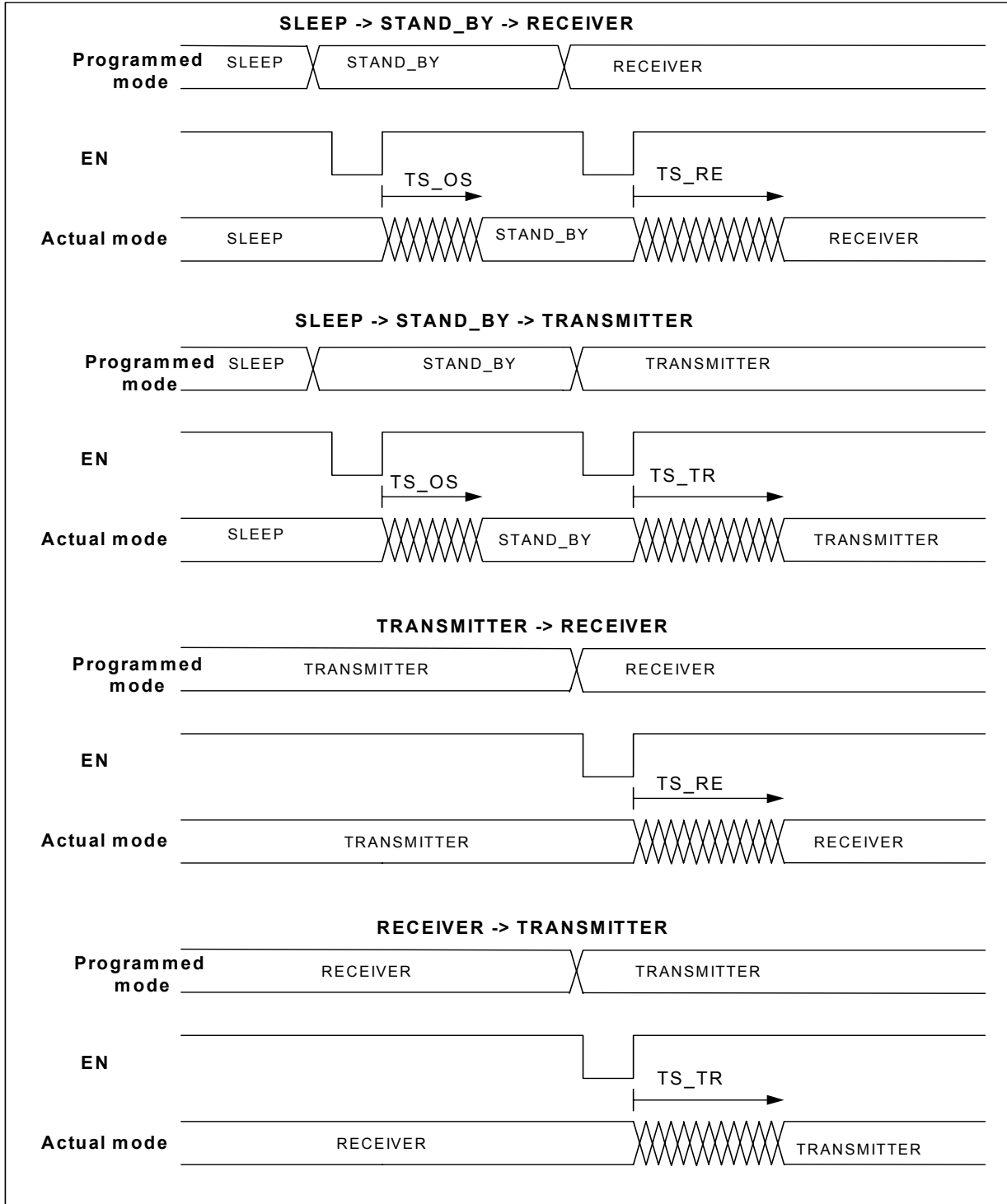
Figure 15. Switching between modes.
