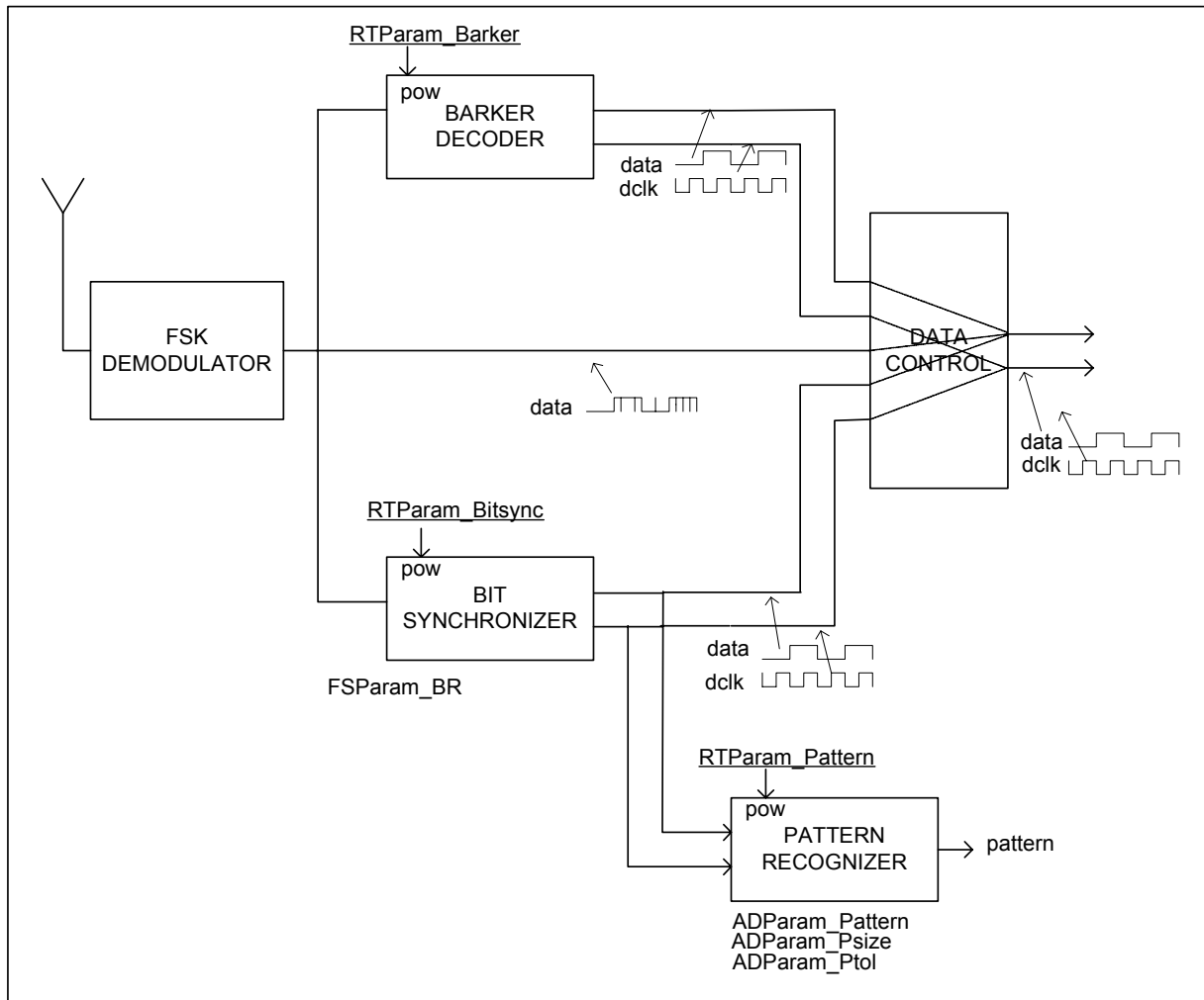
Figure 1 Demodulation architecture.
