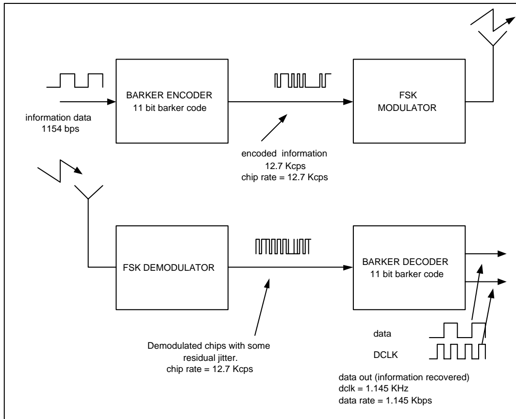
Figure 3. Data encoding decoding channel.
