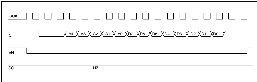
Figure 11 Write sequence into configuration register
