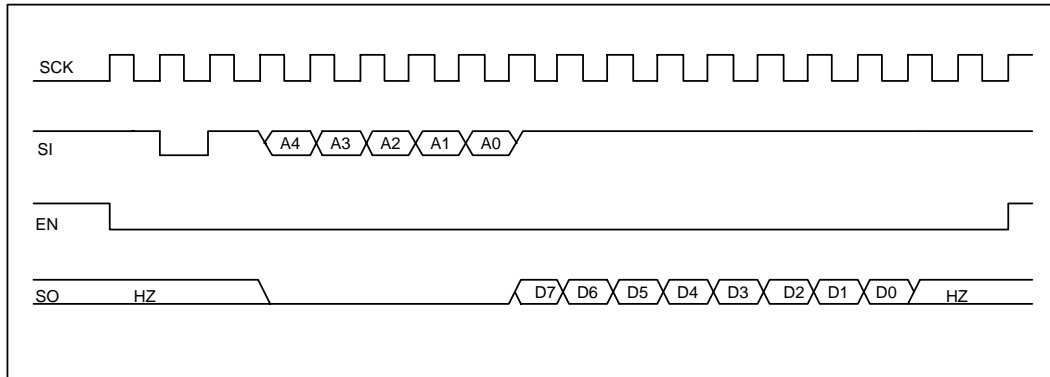
Figure 13 Read sequence of configuration register.
