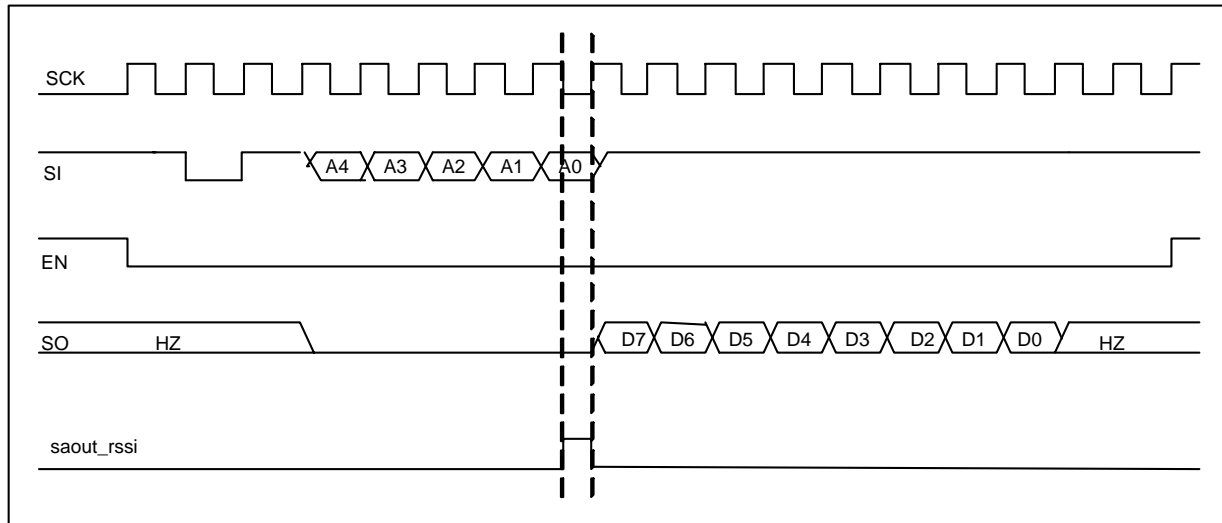
Figure 7. Generation of saout_rssi
