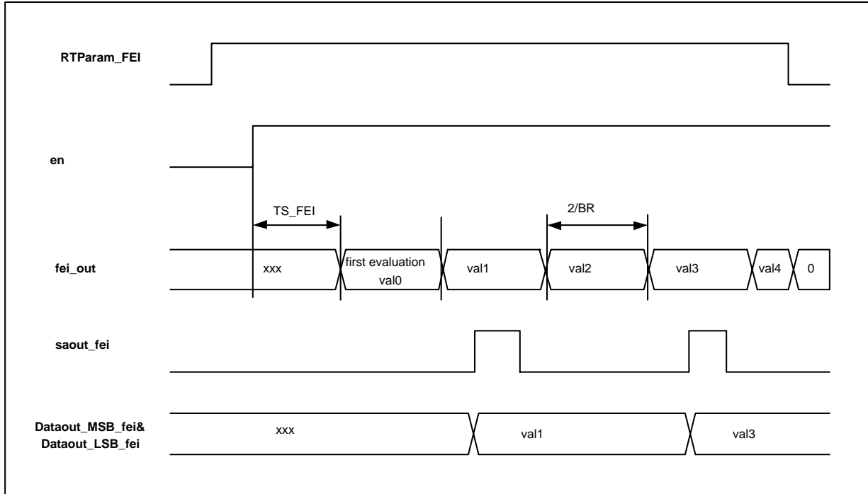
Figure 8 Time diagram of an FEI measurement.
