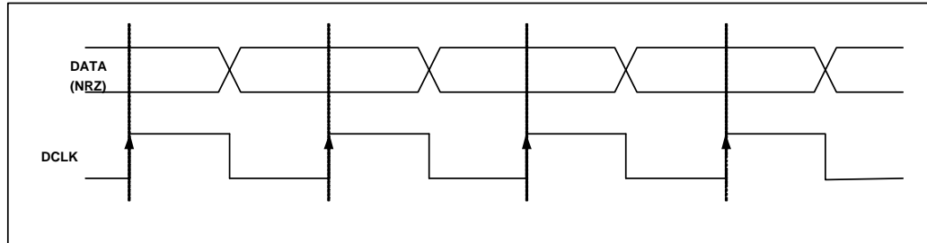
Figure 2. Bit synchronizer timing diagram.
