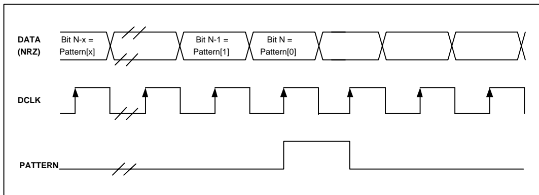
Figure 5. Pattern matching operation.
