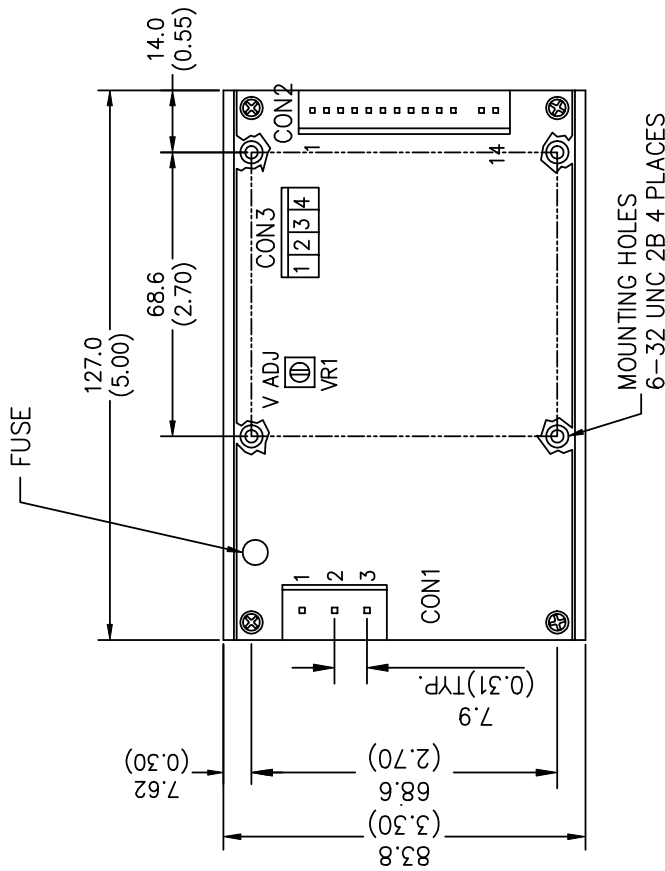
CON2 ( CONNECTORS ) CONFIGURATION FOR V4 ISOLATED
