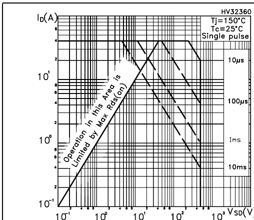
Figure 6. Safe operating area for DPAK / IPAK
