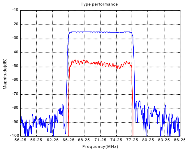
SP71.25 SAW Filter Typical Performance
