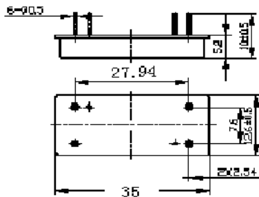
Package Outline
