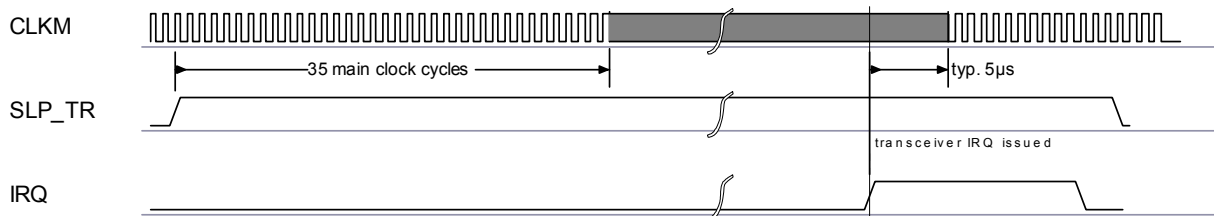
Figure 6-16. Wake-Up Initiated by Radio Transceiver Interrupt
