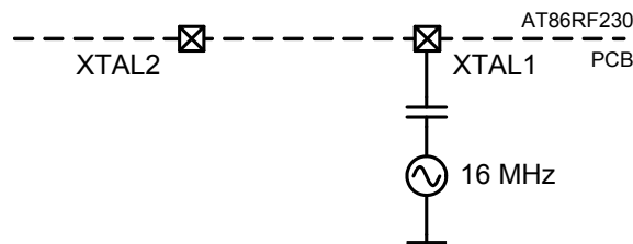
Figure 9-5. Setup for Using an External Frequency Reference
