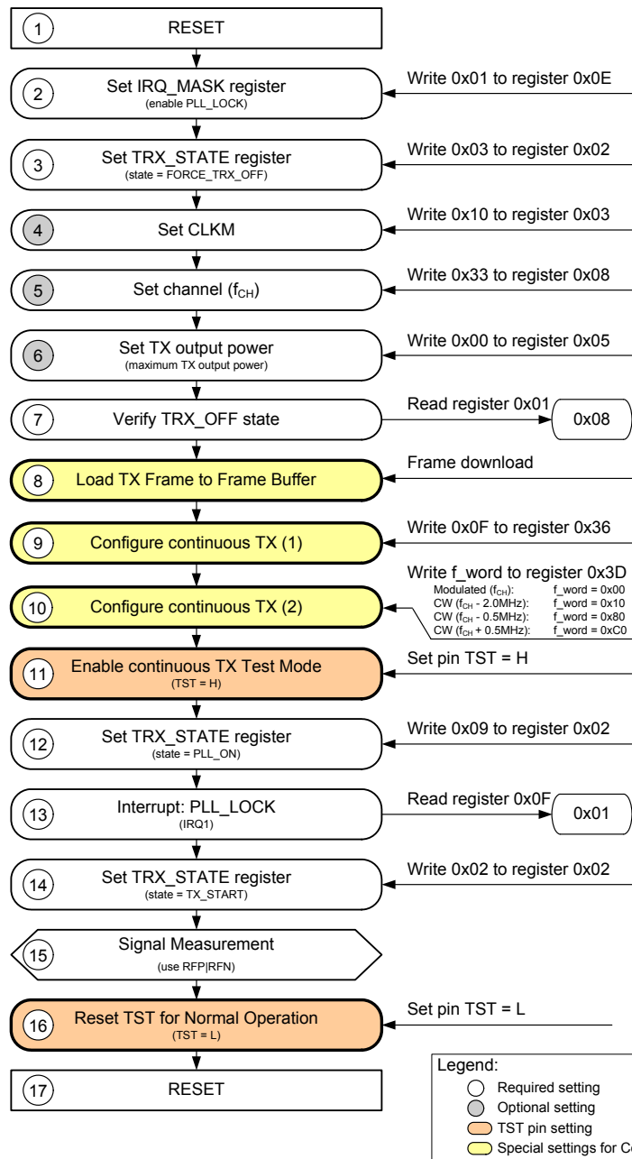
Figure A-1. Programming Sequence - Continuous Transmission
