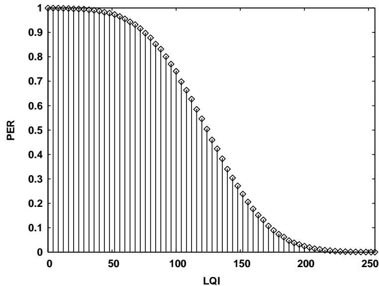
Figure 8-3. Conditional Packet Error Rate versus LQI
