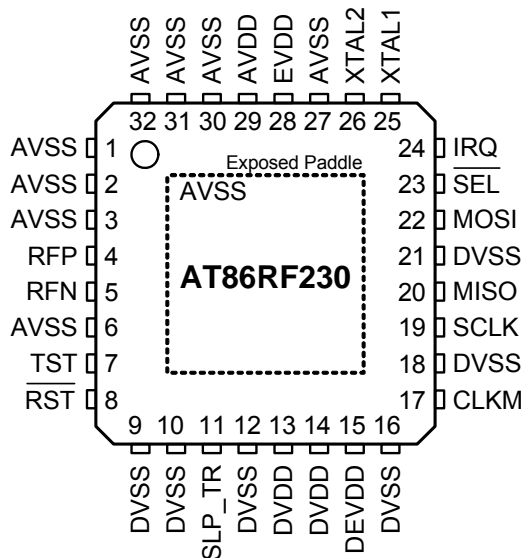
Figure 1-1. AT86RF230 Pin-Out Diagram
