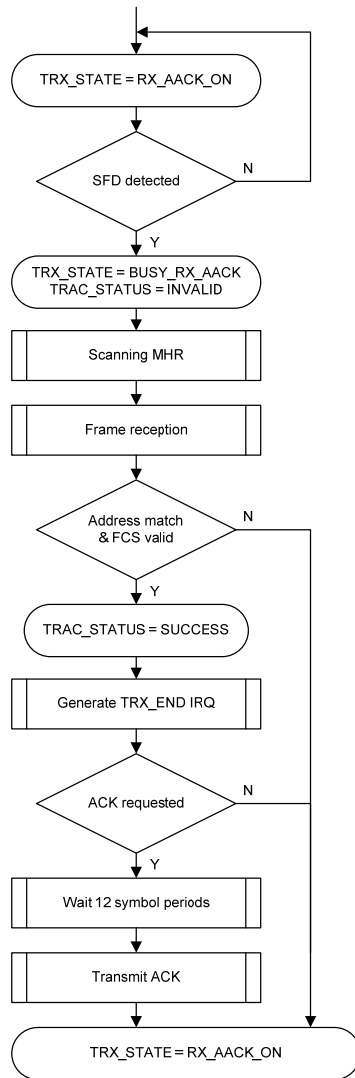
Figure 7-6. Flow Diagram of RX_AACK
