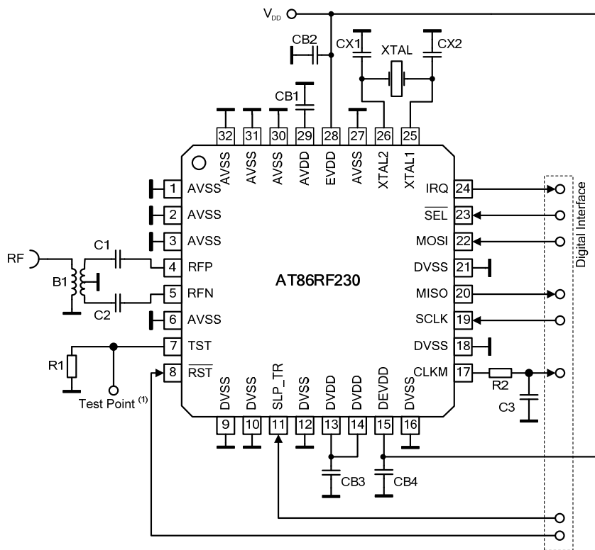
Figure 5-1. Application Circuit Schematic
