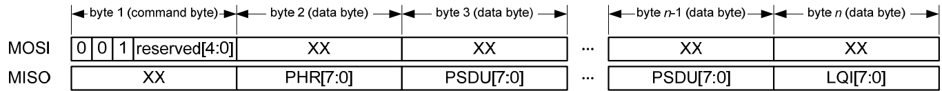
Figure 6-8. Packet Structure - Frame Buffer Read Access
