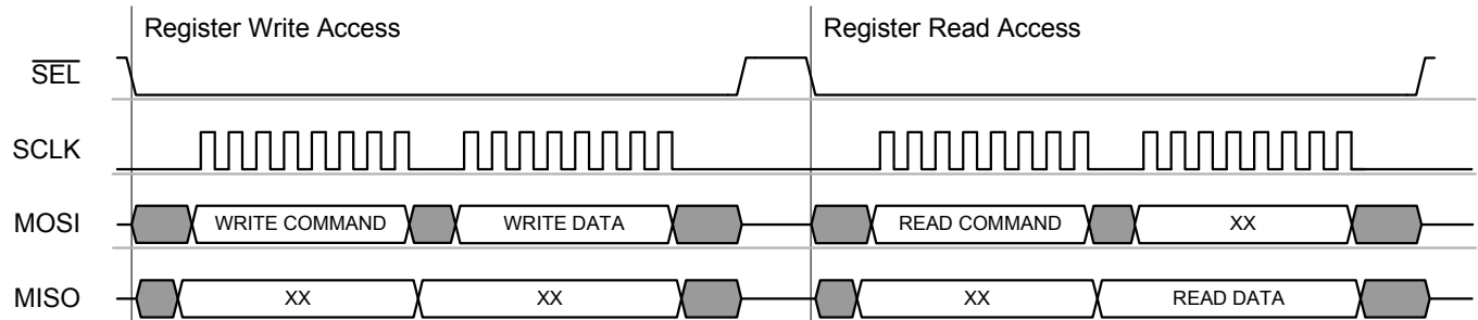
Figure 6-6. Example SPI Sequence - Register Access Mode
