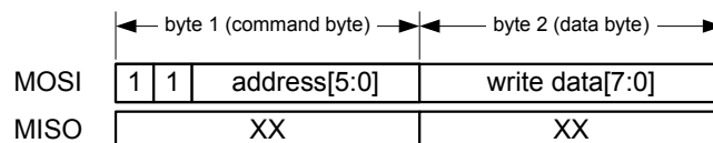
Figure 6-4. Packet Structure – Register Write Access
