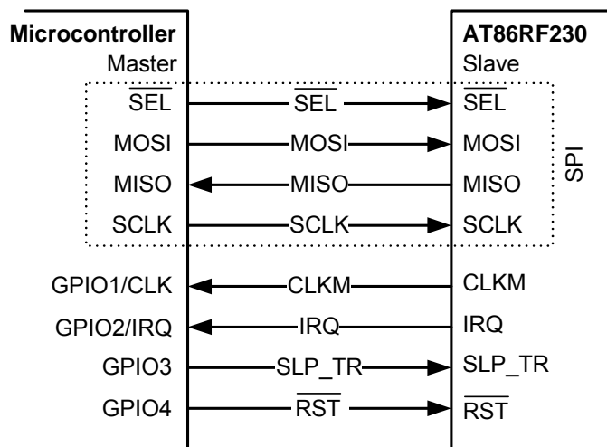
Figure 6-1. Microcontroller to AT86RF230 Interface
