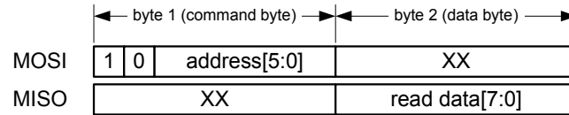
Figure 6-5. Packet Structure – Register Read Access
