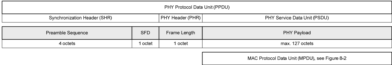
Figure 8-1 IEEE 802.15.4-2003 Frame Format – PHY Layer Frame Structure
