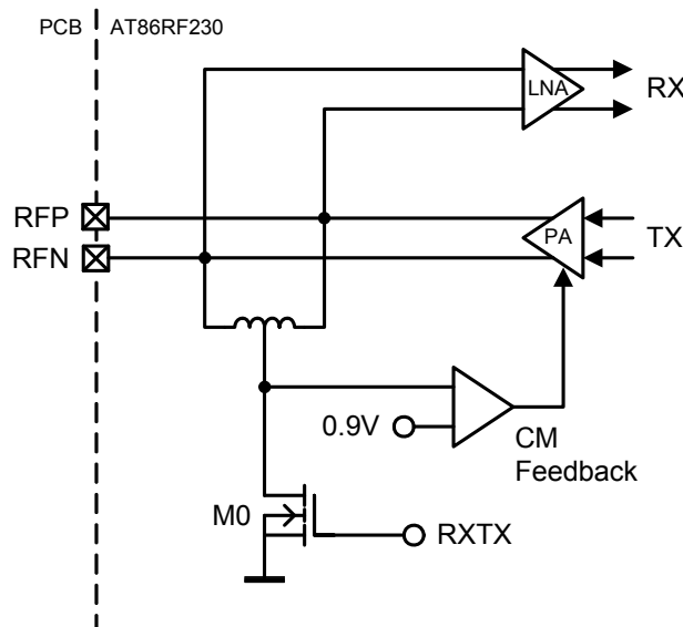
Figure 4-1. Simplified RF Front-End Schematic
