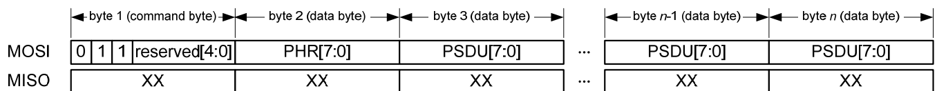
Figure 6-7. Packet Structure - Frame Buffer Write Access
