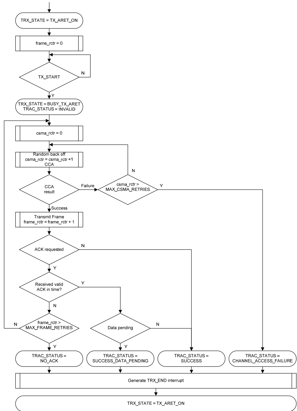
Figure 7-8 Flow Diagram of TX_ARET
