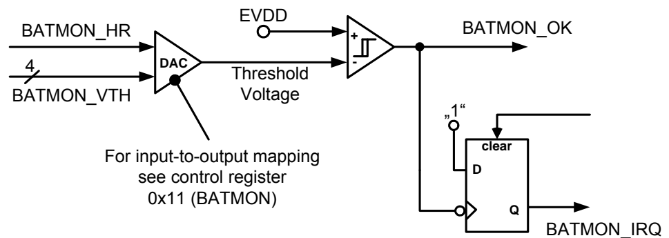
Figure 9-3. Simplified Schematic of BATMON
