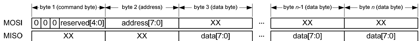
Figure 6-12. Packet Structure - SRAM Read Access
