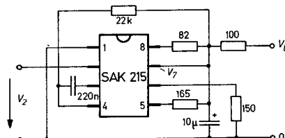
Fig. 3: Test circuit for the characteristics
