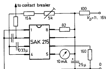
Fig. 2: Block diagram and operating circuit of the SAK215
