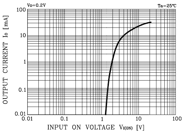
Fig. 1 I_O - V_{I(ON)}
