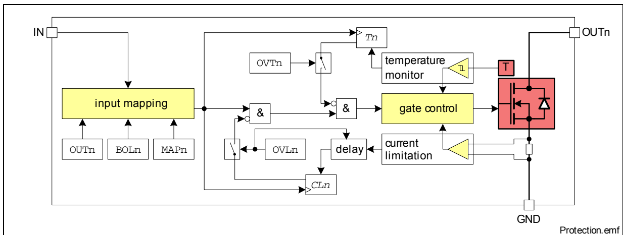
Figure 7 Protective Functions
