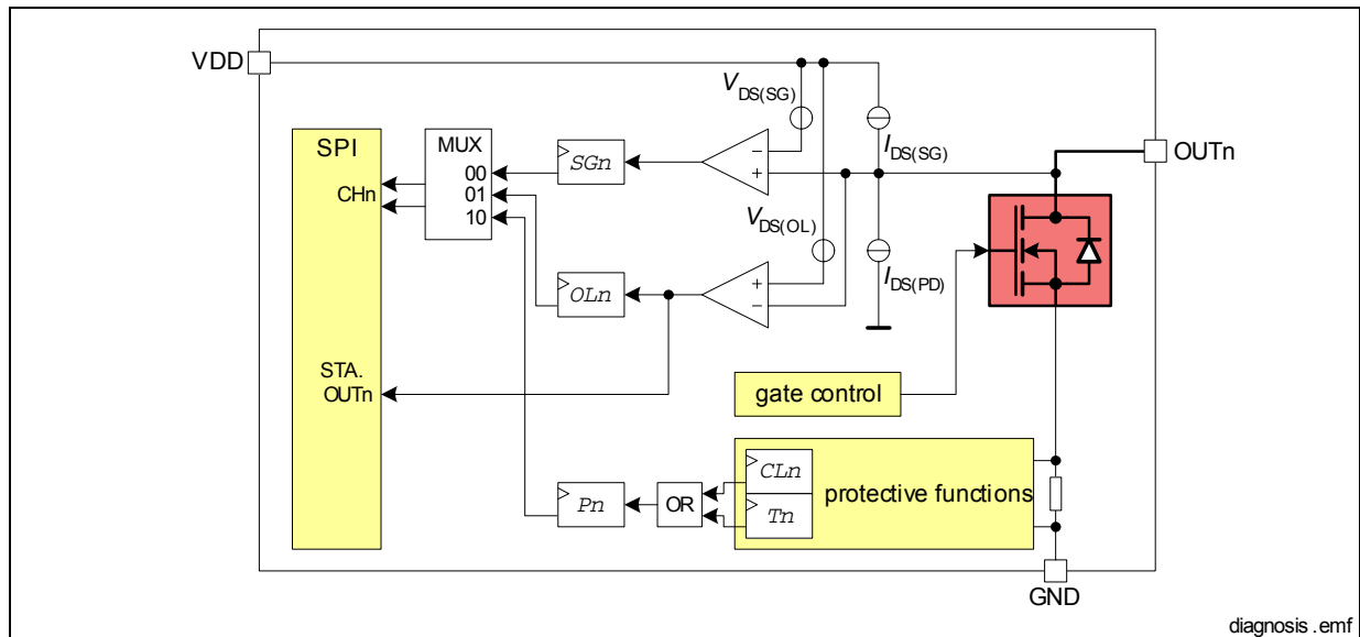
Figure 9 Block Diagram Diagnosis
