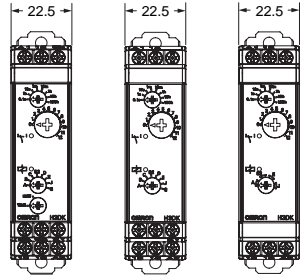
H3DK-M2 H3DK-S2
