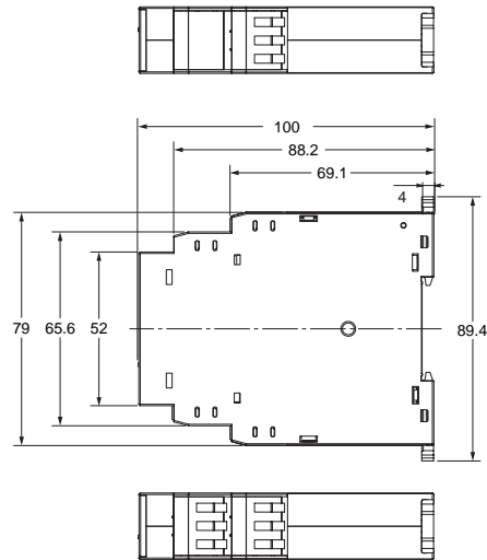
H3DK-S1
