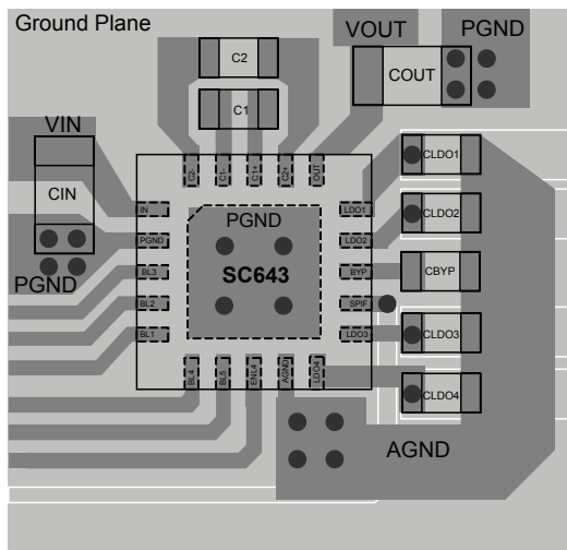
Figure 2 — Recommended PCB Layout
