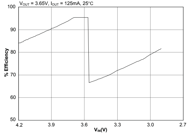
Backlight Efficiency (5 LEDs) — 25mA Each
