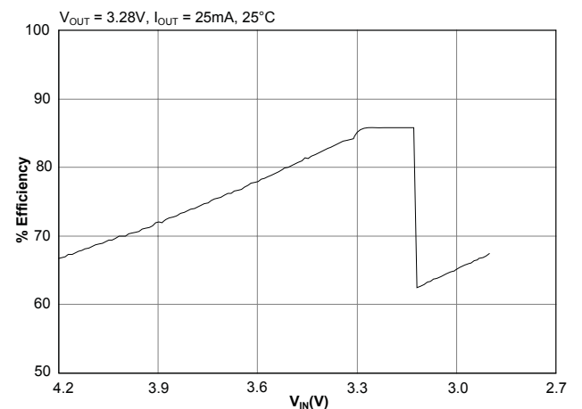
Backlight Efficiency (5 LEDs) — 5.0mA Each
