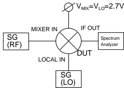
Conversion Gain Measuring Block Diagram
