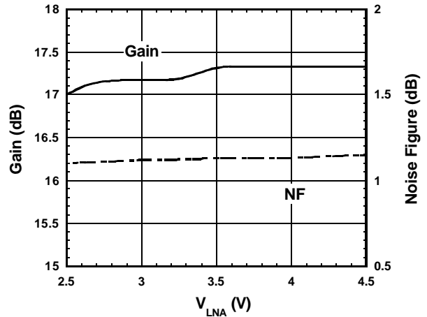
Gain, NF vs. V_{LNA}
