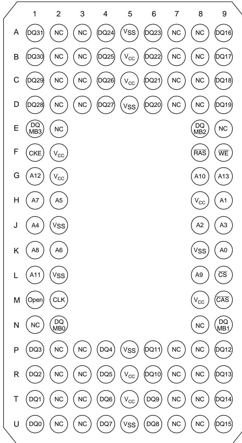
(Top view)
