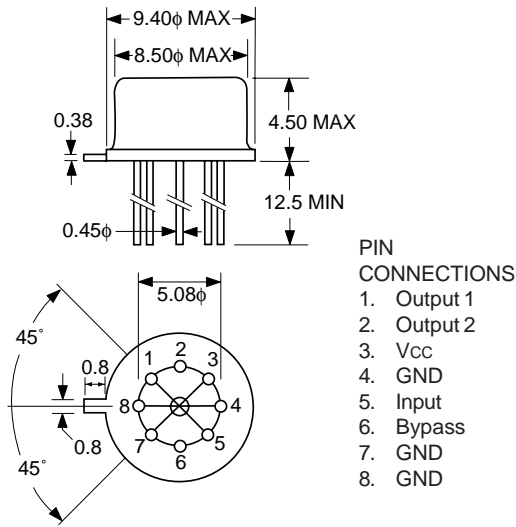
UPB582A PACKAGE OUTLINE A08
