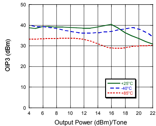
Output IP3
