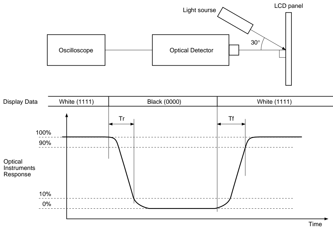
Fig. 3. Measurement system-3
