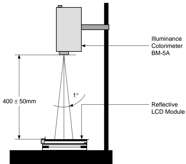
(a) The apparatus for luminance measurement
