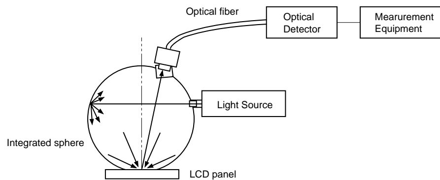
Fig. 2. Measurement system-2
