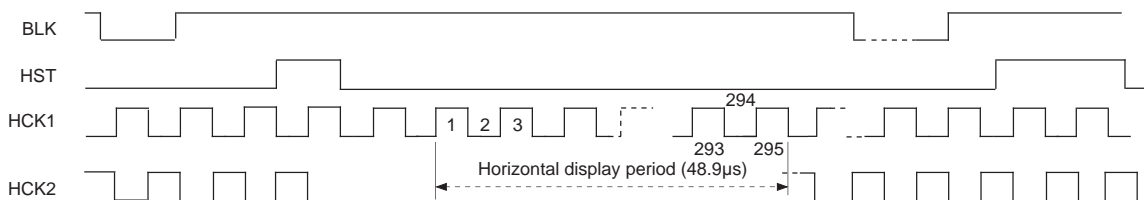
(3) Horizontal display period (RGT: high level)
