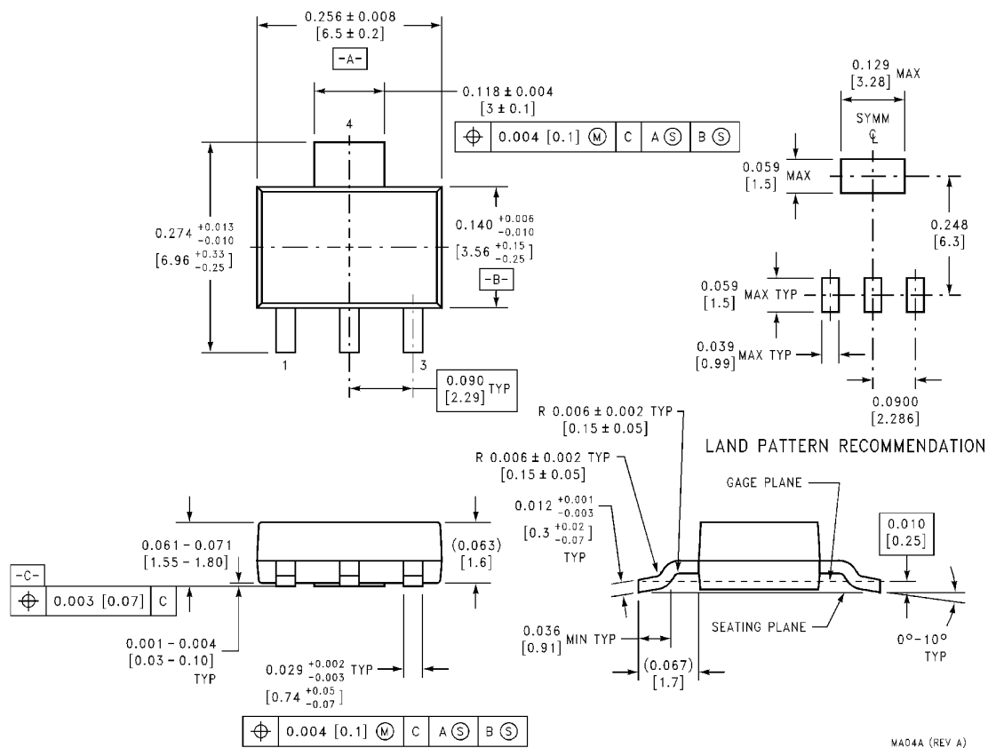
NSC Package Number MA04A
