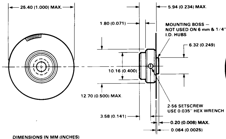
Figure 4. HEDS-5120 Codewheel.
