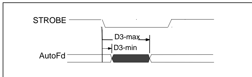
Figure 43 - Serial Interface Output Delay Timing
