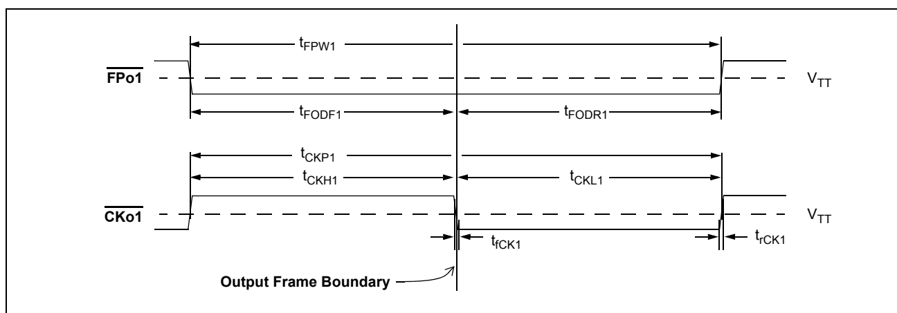
Figure 41 - \overline{\text{FPo1}} and \overline{\text{CKo1}} Timing Diagram
