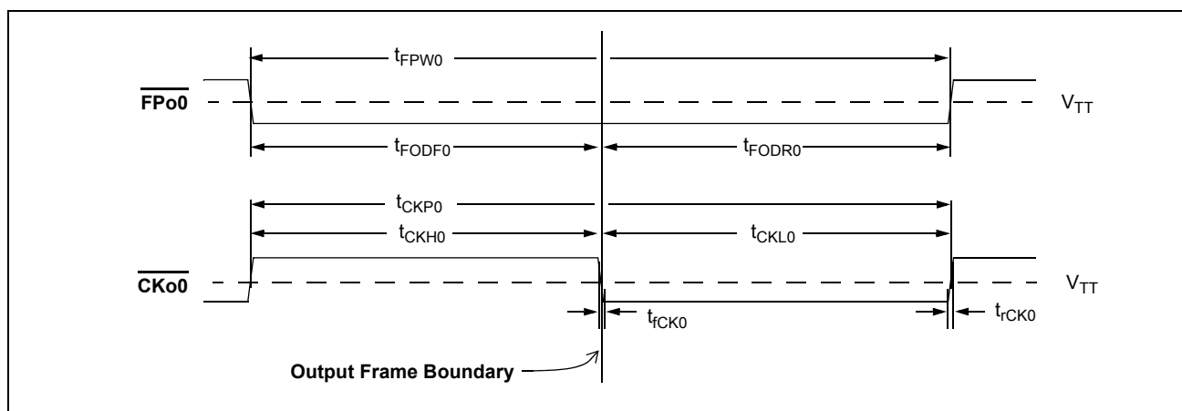
Figure 40 - \overline{\text{FPo0}} and \overline{\text{CKo0}} Timing Diagram
