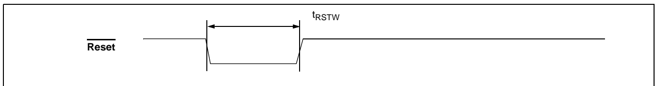
Figure 50 - Reset Pin Timing Diagram
