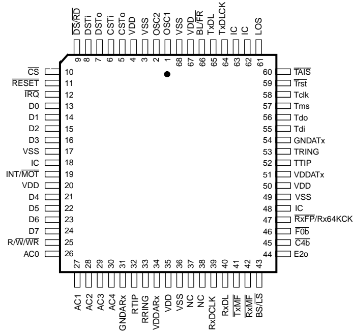
68 PIN PLCC
