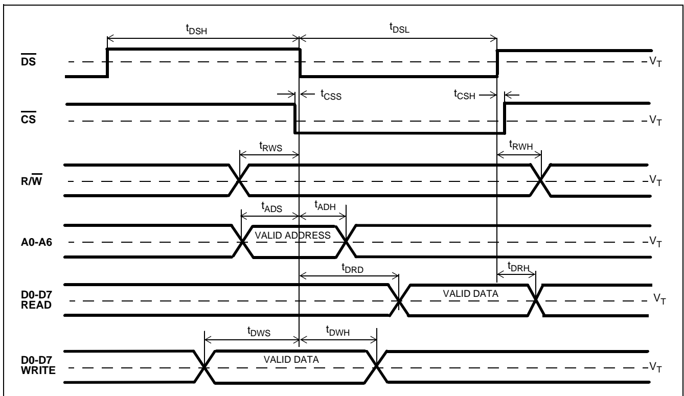
Figure 17 - Microport Timing
