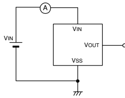
Circuit 2
