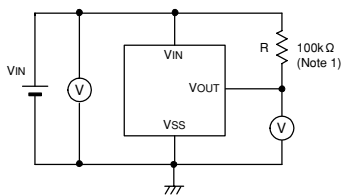
Circuit 1
