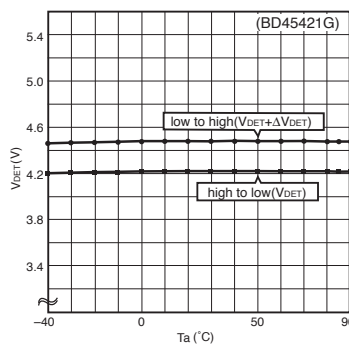
Detection voltage
