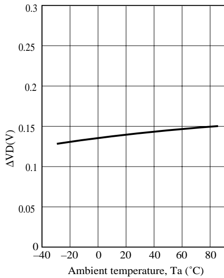
Figure 8.a. \Delta VD Temperature Characteristic (Rank Q)
