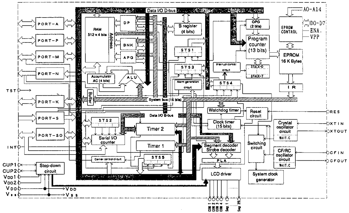
LC58E7008 System Block Diagram
