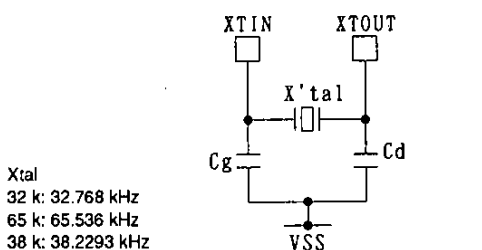
Figure 1-(1) Specified Oscillator Circuit (XT pin)
