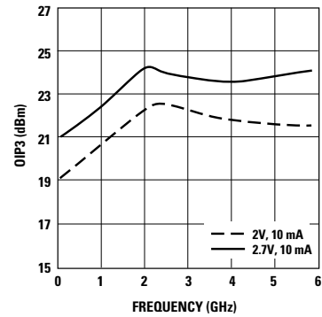
Figure 8. OIP3 vs. Bias over Frequency. [1]
