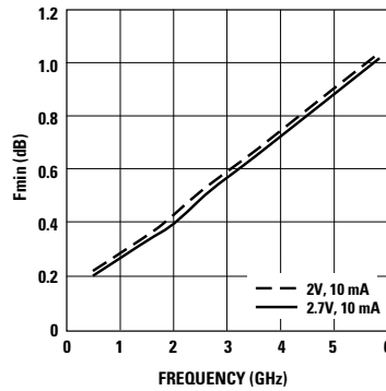
Figure 7. Fmin vs. Frequency and Bias.
