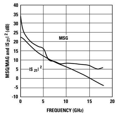
Figure 27. MSG/MAG and IS_{21}^2 vs. Frequency at 2V, 15 mA.
