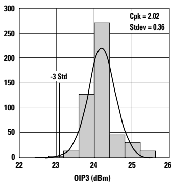
Figure 2. OIP3 @ 2.7V, 10 mA. LSL = 22.0, Nominal = 24.2
