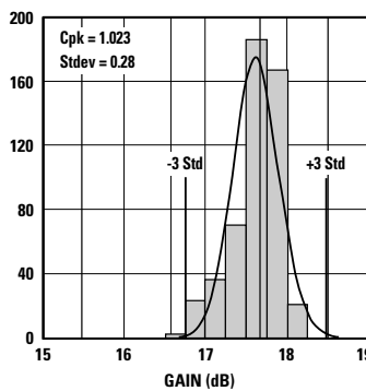
Figure 3. Gain @ 2.7V, 10 mA. USL = 18.5, LSL = 15.5, Nominal = 17.7
