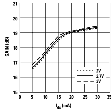
Figure 11. Gain vs. I_{ds} and V_{ds} at 2 GHz. [1]
