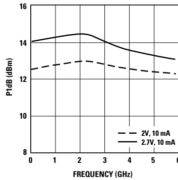
Figure 10. P1dB vs. Bias over Frequency. [1,2]
