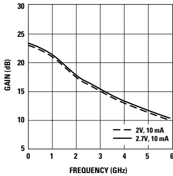
Figure 6. Gain vs. Bias over Frequency. [1]
