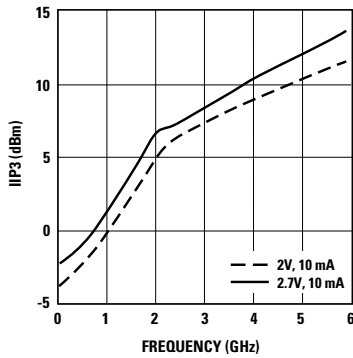
Figure 9. IIP3 vs. Bias over Frequency. [1]
