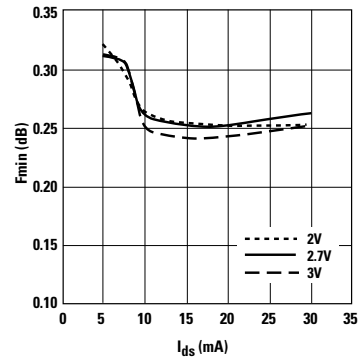
Figure 17. F_{min} vs. I_{ds} and V_{ds} at 900 MHz.
