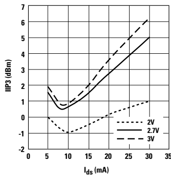
Figure 19. IIP3 vs. I_{ds} and V_{ds} at 900 MHz. [1]
