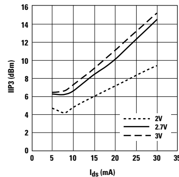
Figure 14. IIP3 vs. I_{ds} and V_{ds} at 2 GHz. [1]
