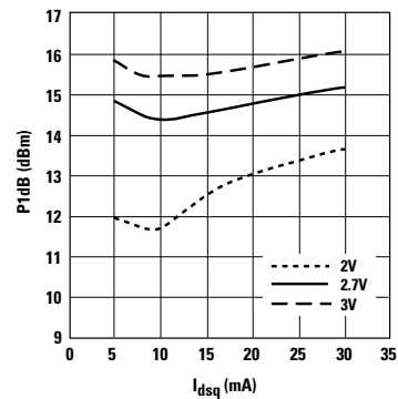
Figure 20. P1dB vs. I_{dsq} and V_{ds} at 900 MHz. [1,2]
