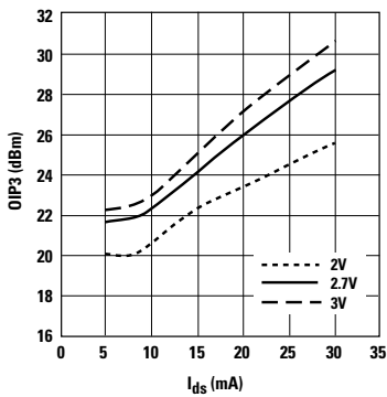
Figure 18. OIP3 vs. I_{ds} and V_{ds} at 900 MHz. [1]
