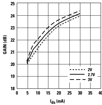
Figure 16. Gain vs. I_{ds} and V_{ds} at 900 MHz. [1]
