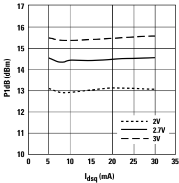
Figure 15. P1dB vs. I_{dsq} and V_{ds} at 2 GHz. [1,2]
