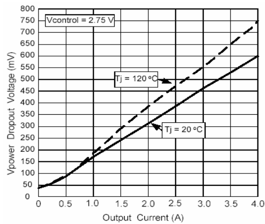
Vpower Dropout Voltage vs Output Current
