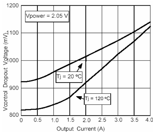
Vcontrol Dropout Voltage vs Output Current
