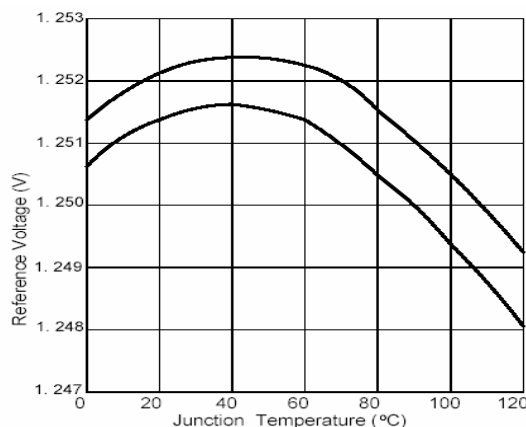
Reference Voltage vs Junction Temperature
