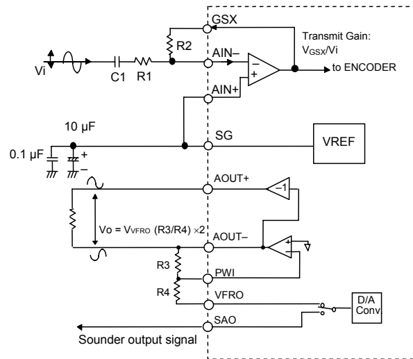
Figure 1 Analog Input/Output Interface
