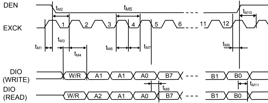
Figure 5 Serial Control Port Interface
