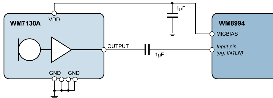
Figure 2 WM7130A Silicon Microphone Single-ended Connection to WM8994
