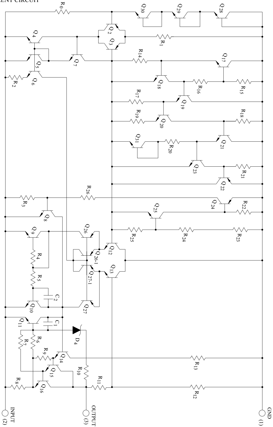
EQUIVALENT CIRCUIT
