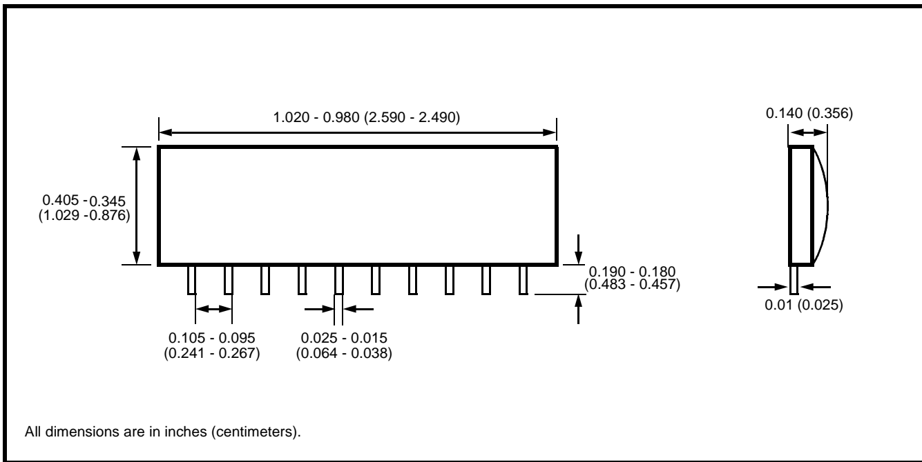
Figure 4 - Mechanical Data
