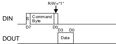
Figure 14. Setup Command Read
