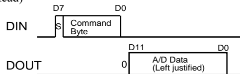
Figure 8. Single Read (External Clock Mode)
