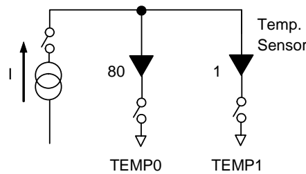
Figure 6. Temperature Measurement
