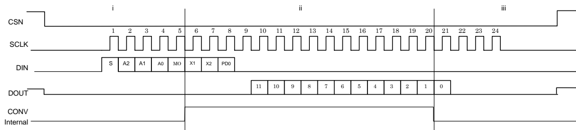
Figure 23. PENIRQN Functional Timing Chart
