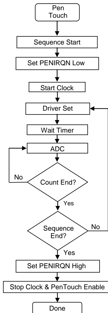
Figure 19. Internal Clock Mode Control Flowchart
