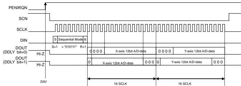
Figure 21. Internal Clock Mode Control Sequence (X-Y Scan: SEQM bits = “001”) (Data Available → A/D Data Read)
