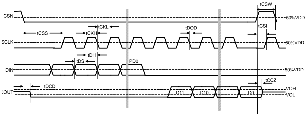
Figure 2. Timing Diagram
