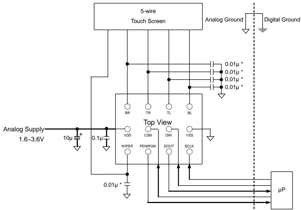
Figure 25. Typical Connection Diagram
