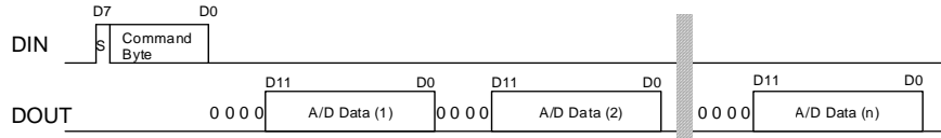
Figure 9. Continuous Read (External Clock Mode: DDLY bit = "0")
