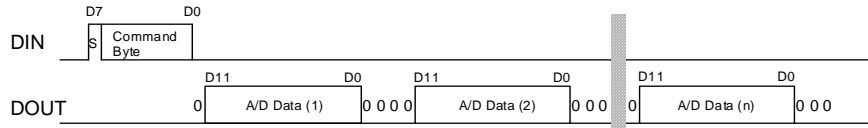
Figure 10. Continuous Read (External Clock Mode: DDLY bit = "1")
