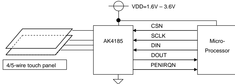
Figure 7. Digital I/F
