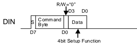
Figure 13. Setup Command Write
