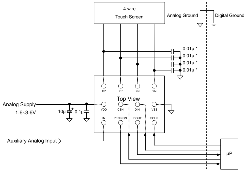
Figure 24. Typical Connection Diagram
