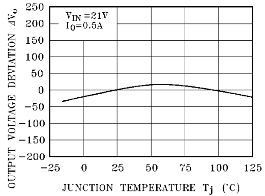
Fig.5-4 T_j - \Delta V_o (KIA78R15)
