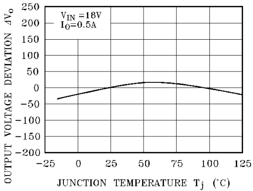
Fig.5-3 T_j - \Delta V_o (KIA78R12)
