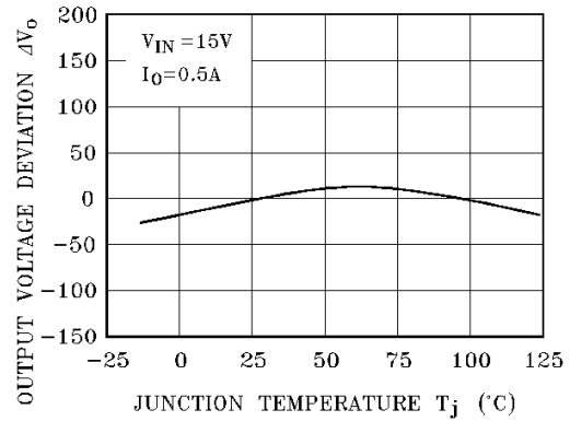
Fig.5-2 T_j - \Delta V_o (KIA78R09)
