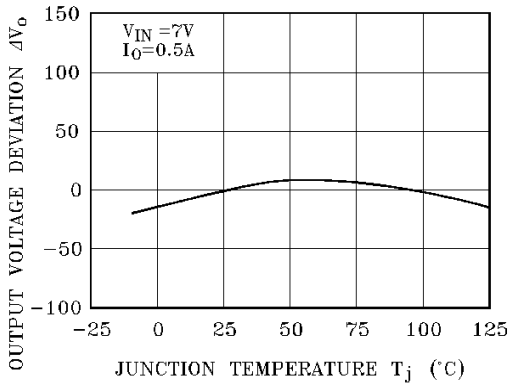
Fig.5-1 T_j - \Delta V_o (KIA78R05)
