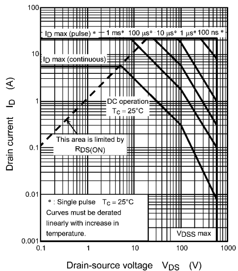
Fig. 8.17 Safe Operating Area (Guaranteed Maximum)
